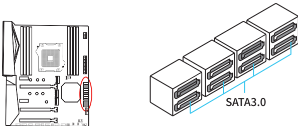
2 -11 SATA Interface
