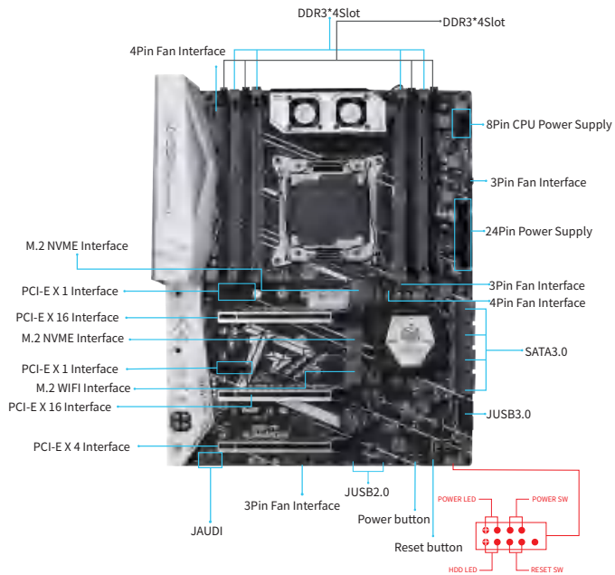
1-1 X99-TF Motherboard Illustration
